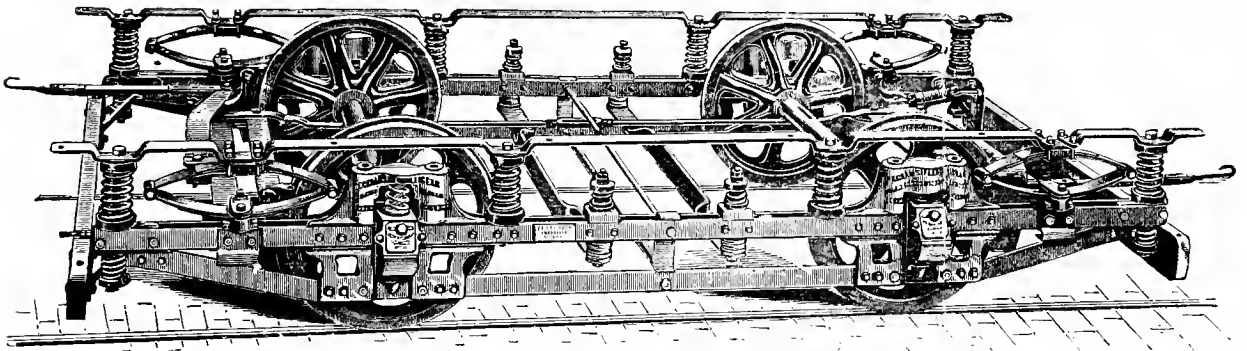
Fig. 5670. TRUCK FOR STREET-CARS. THE PECKHAM STANDARD.
